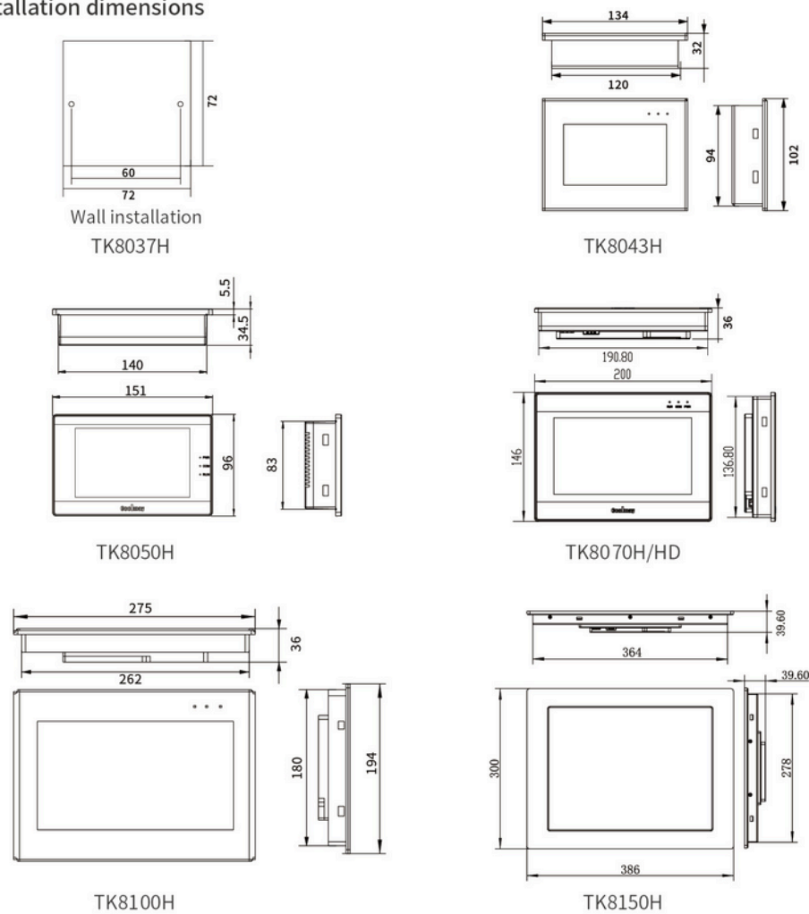
Figure 1 Installation dimensions diagram
